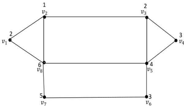
Figure 1. \gamma_{\chi}^d(G) = 6
