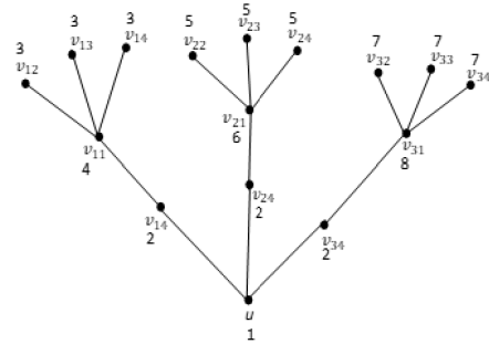
Figure 5. \gamma_{\chi}^d(B_{3,4}) = 8
